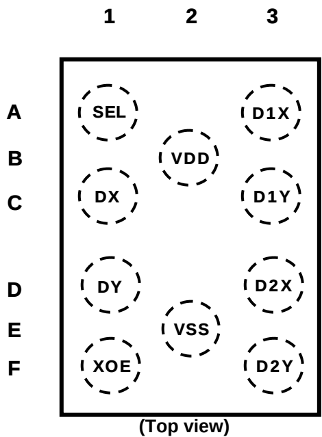
Fig.2 Pin Assignment
