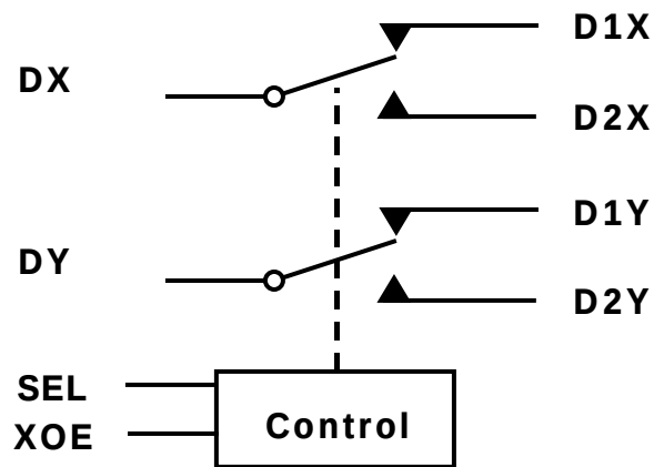
Fig.3 Bus switch symbol
